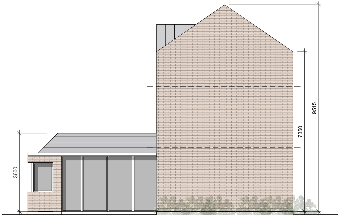
GABLE ELEVATION HOUSE No.64
